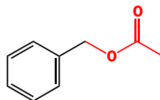
benzyl acetate
