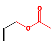
allyl acetate
