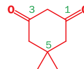
"dimedone" 5,5-dimethylcyclohexane-1,3-dione
